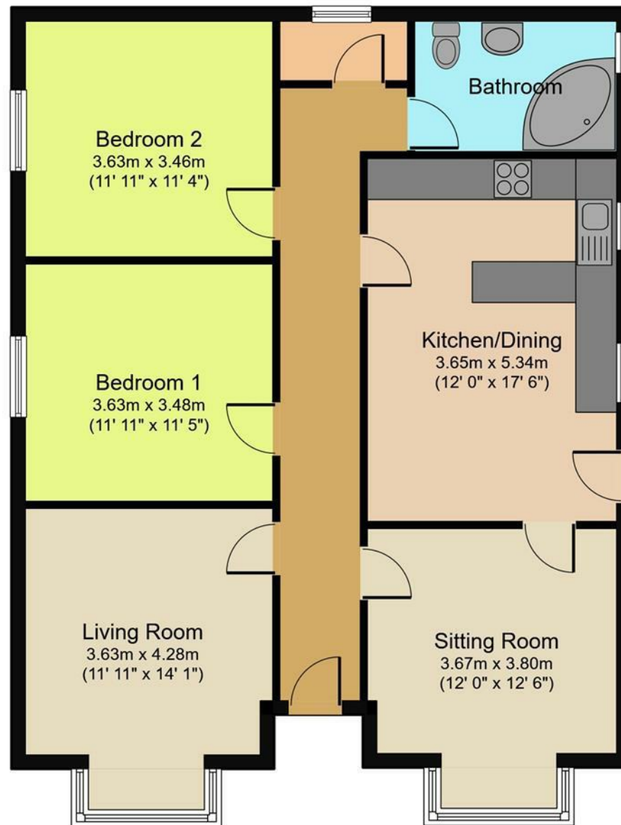
Ground Floor
